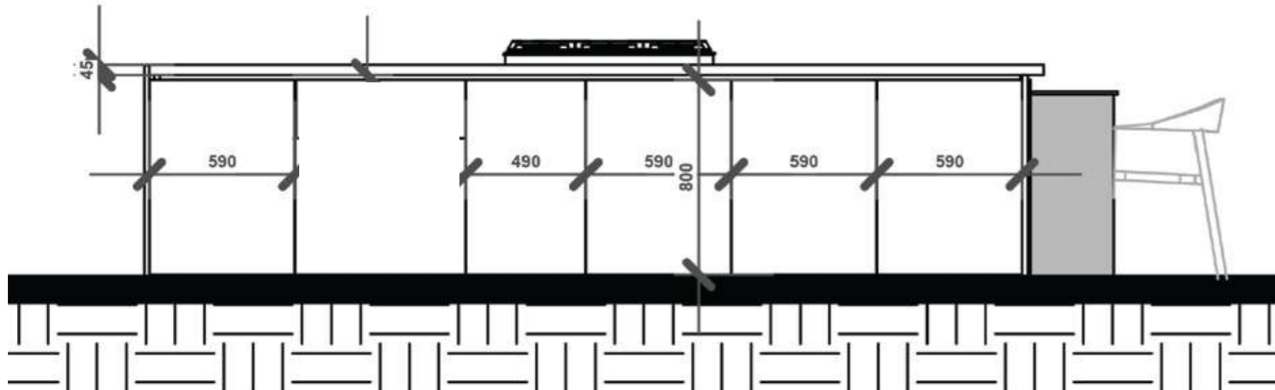
SECTIONAL ELEVATION OF CUPBOARDS ON THE STANDING ISLAND
