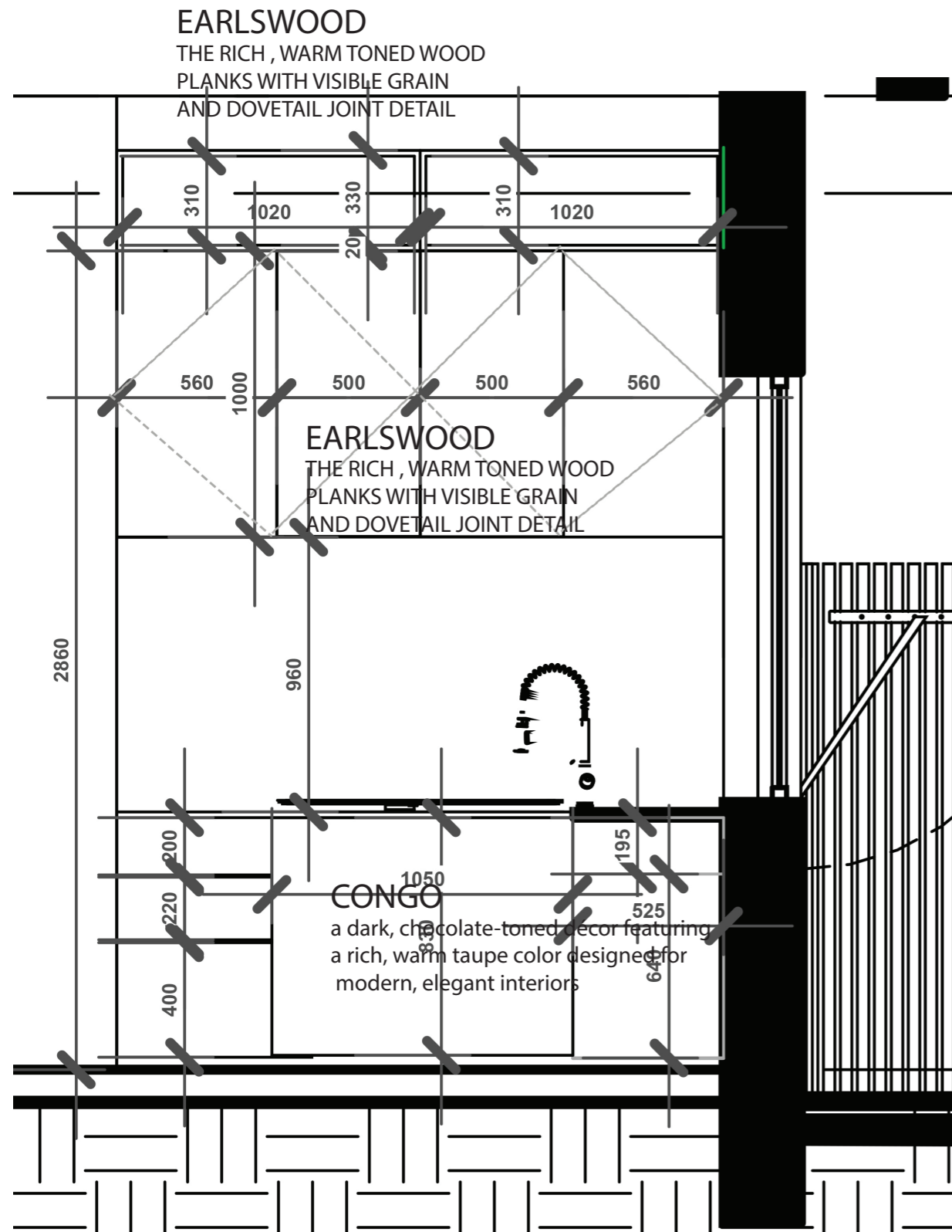
FRONT SECTION
