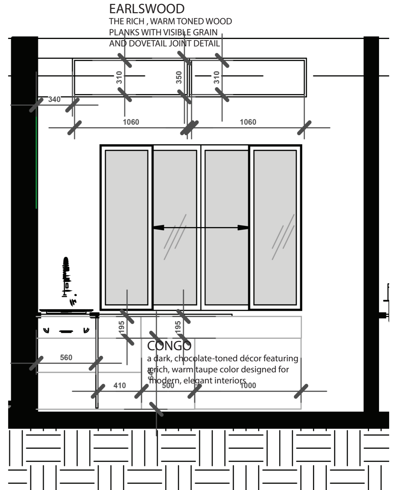
SIDE SECTION
