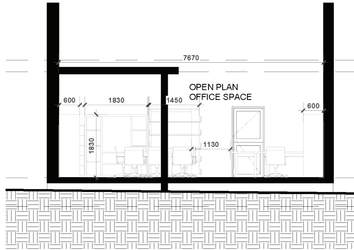
NEW PROPOSED OFFICE SECTION B-B
