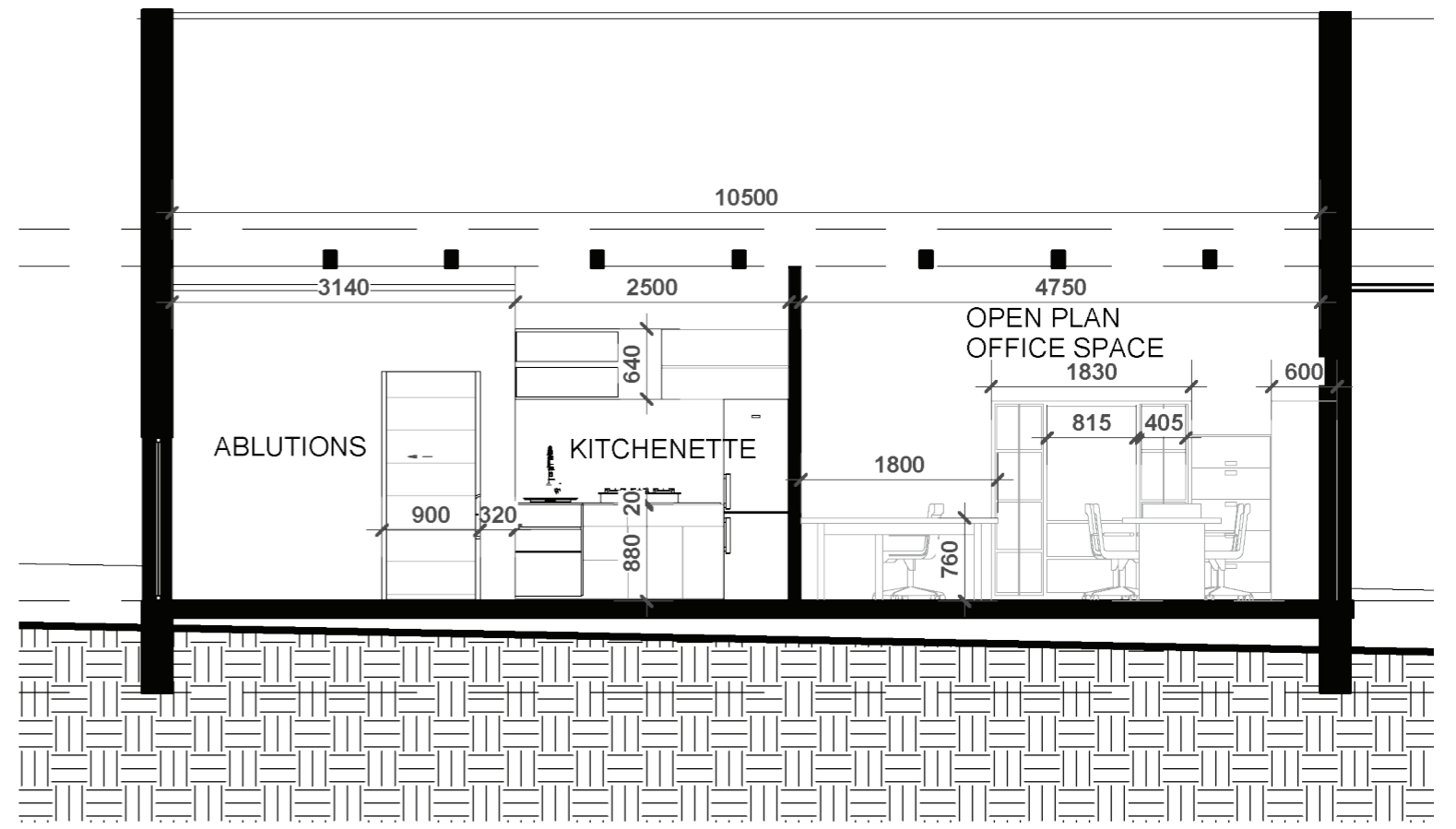
NEW PROPOSED OFFICE SECTION A-A
